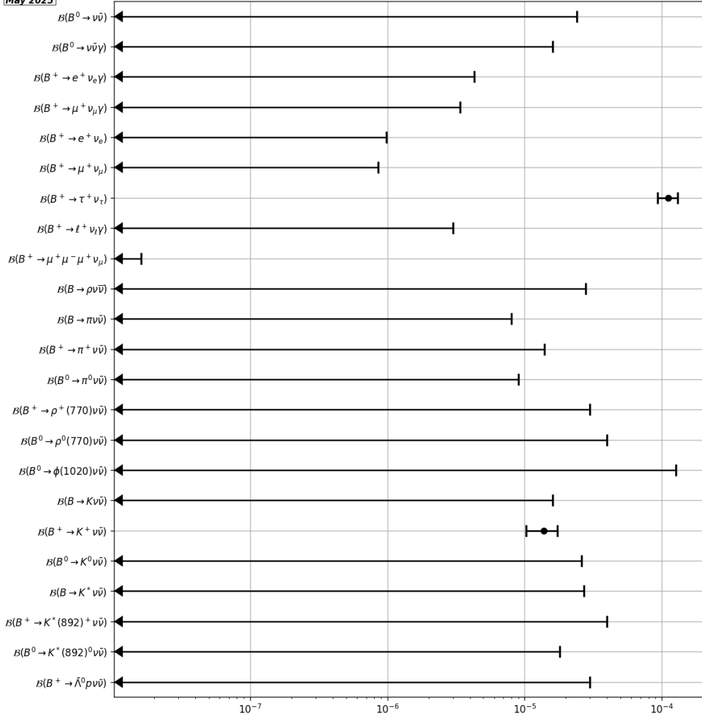
Figure 13: Branching fractions of charmless B decays with neutrinos.
