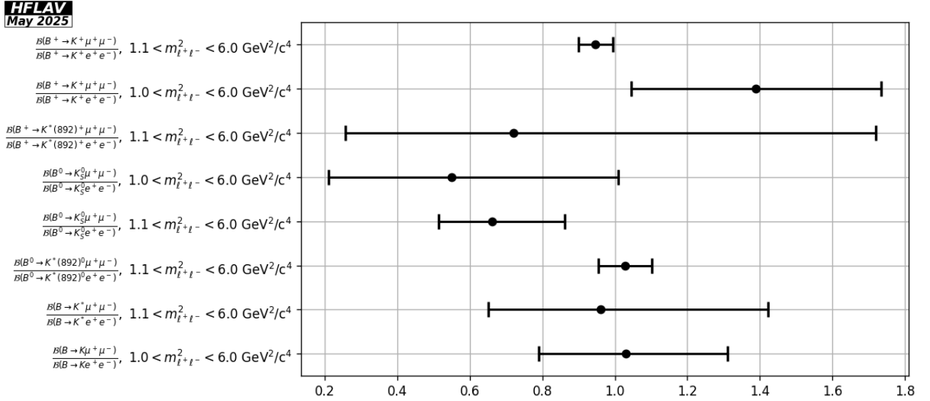
Figure 10: Compilation of R_K^{(*)} ratios in the low dilepton invariant-mass region. These are ratios between branching fractions of B -meson decays to K^{(*)} \mu^+ \mu^- and K^{(*)} e^+ e^- , which provide information on lepton universality.
