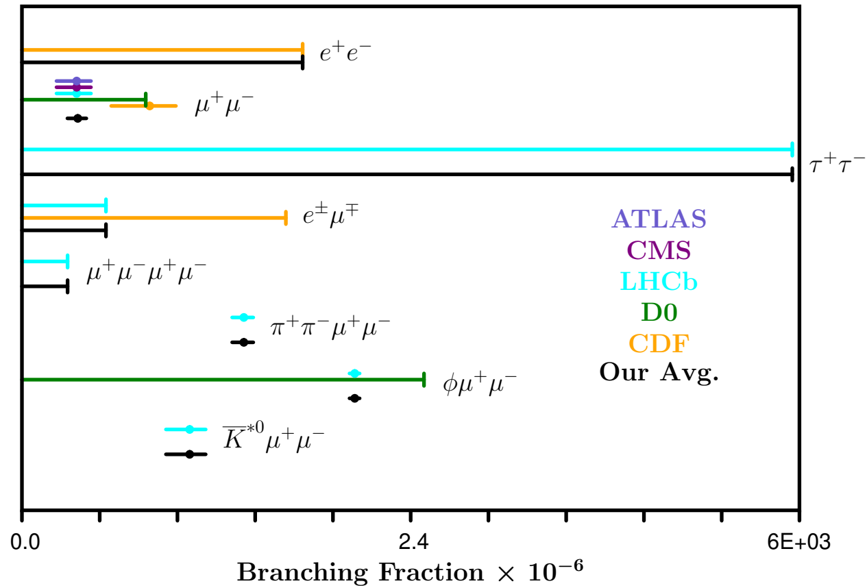
Branching Fractions of Charmless Leptonic B_s Decays
