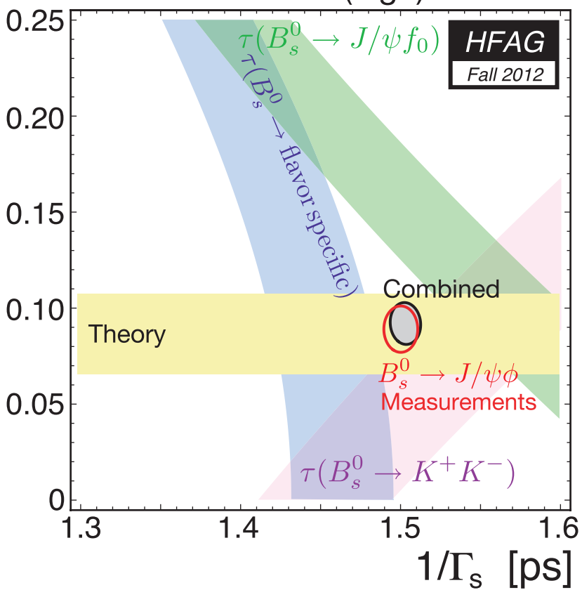
Contours of \Delta(\log L) = 0.5
