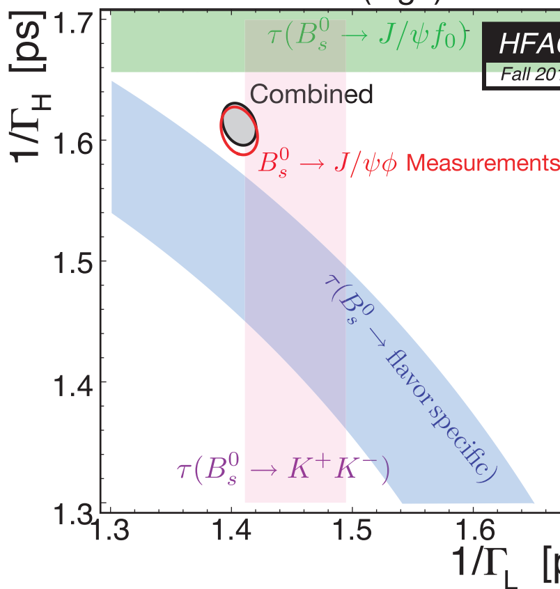
Contours of \Delta(\log L) = 0.5
